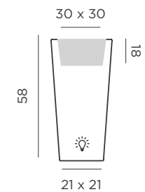
Dimensions (cm)
