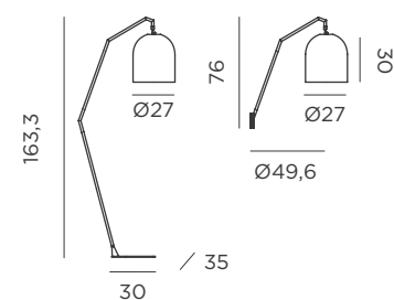
Dimensions (cm)
