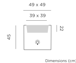
Dimensions (cm)
