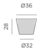
Dimensions (cm)
