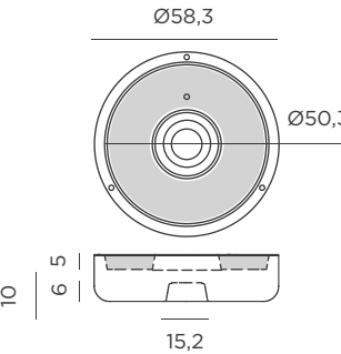
Dimensions (cm)
