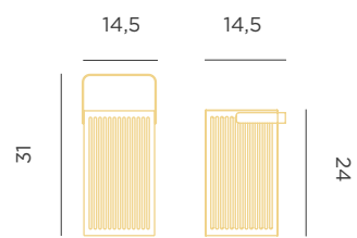
Dimensions (cm)
