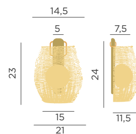
Dimensions (cm)
