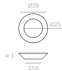
Dimensions (cm)
