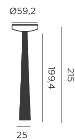
Dimensions (cm)
