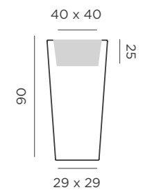
Dimensions (cm)
