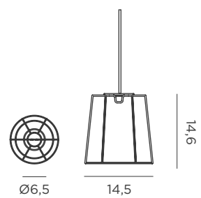
Dimensions (cm)
