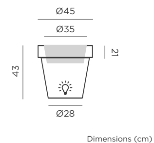
Dimensions (cm)
