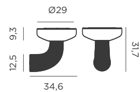
Dimensions (cm)
