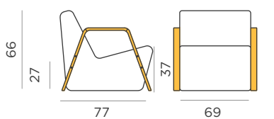
Dimensions (cm)
