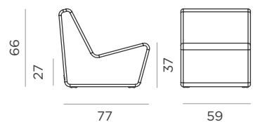
Dimensions (cm)
