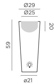
Dimensions (cm)
