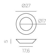
Dimensions (cm)
