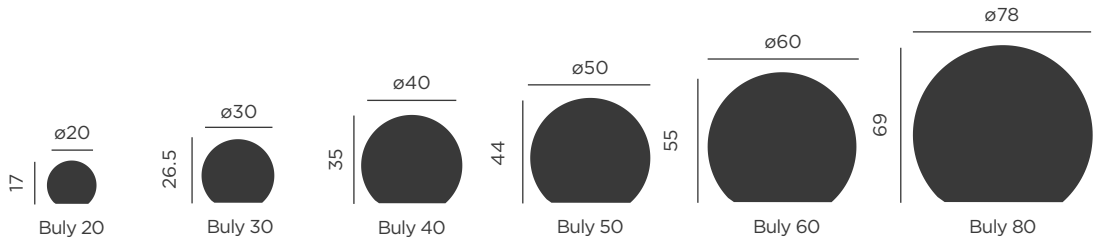
Dimensions (cm)
