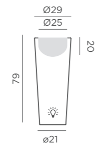
Dimensions (cm)
