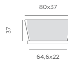
Dimensions (cm)
