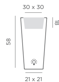
Dimensions (cm)
