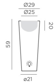
Dimensions (cm)
