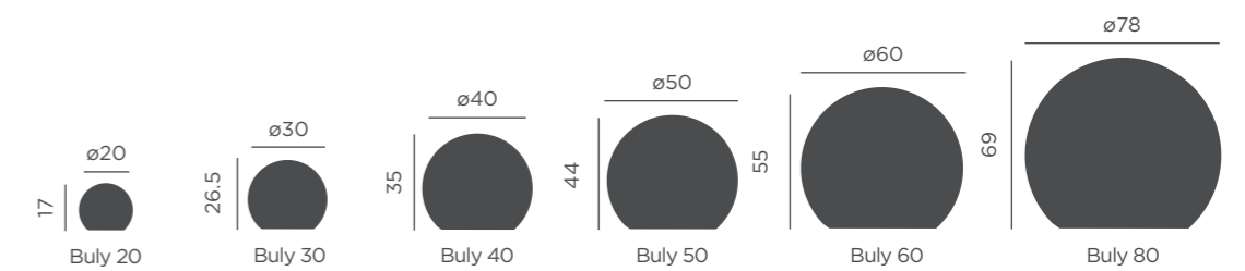
Dimensions (cm)
