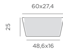
Dimensions (cm)
