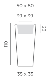
Dimensions (cm)
