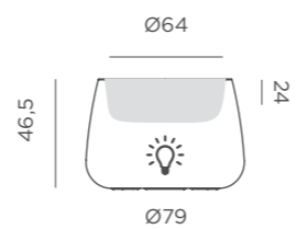
Dimensions (cm)
